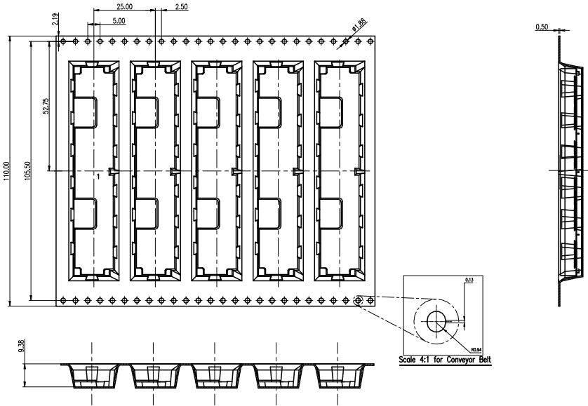
Packaging Carrier Tape Diagram(H=3.05)
