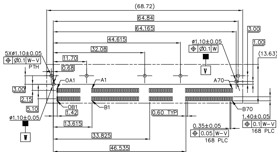
RECOMMENDED 4C+ FOOTPRINT
